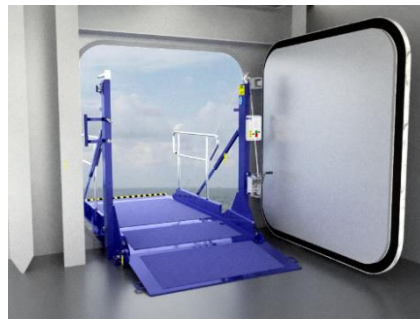
Alt.1 – Quick Lock in deck
